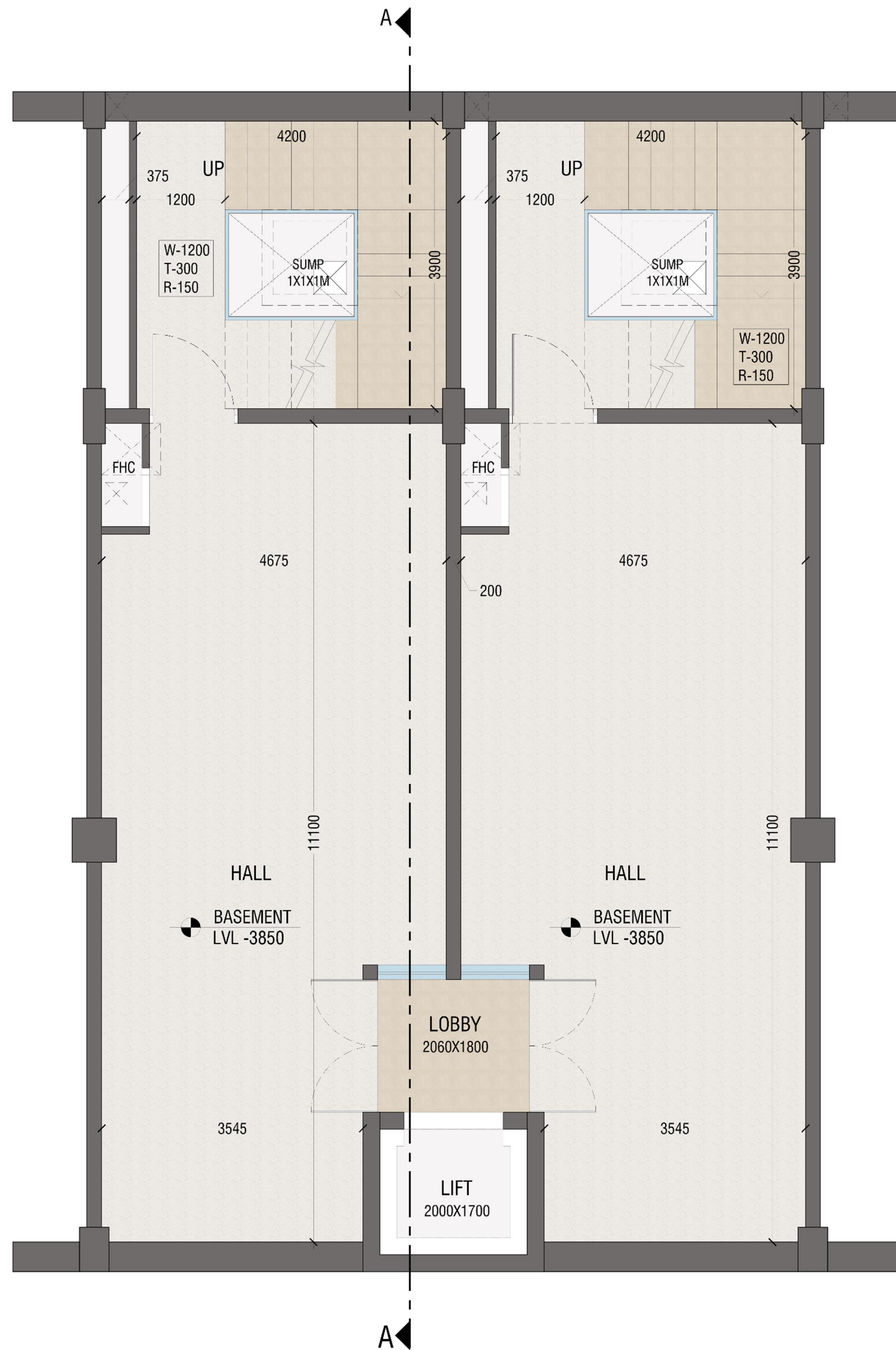
BASEMENT
